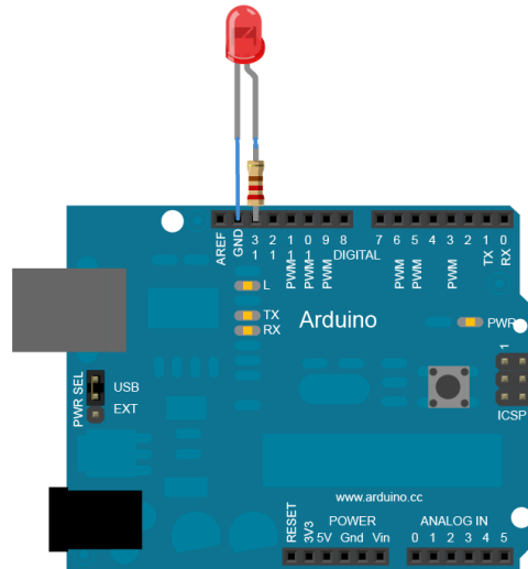
Figure sette.2 An Arduino board with a red LED connected to pin 13 through a 220 \Omega resistor.
