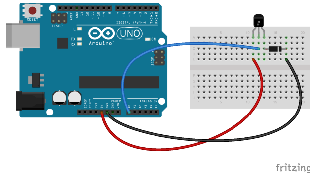
Figure otto.3 Using an LM35 temperature sensor with a forward biased silicon diode, to read negative temperatures.
