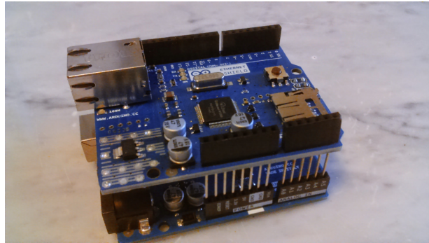
Figure sei.2 An Arduino board with an Ethernet shield mounted on it.
