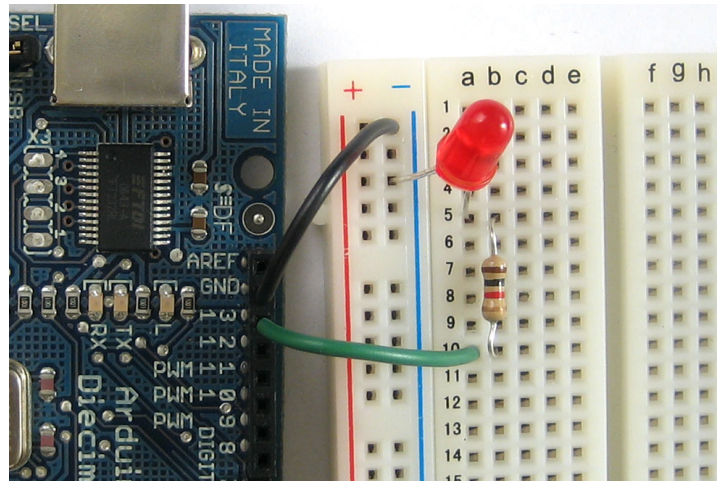
Figure sette.3 An Arduino board with a red LED connected to pin 13 through a 100 \Omega resistor.
