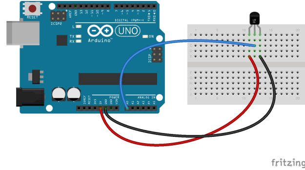
Figure otto.2 Using an LM35 temperature sensor with Arduino.
